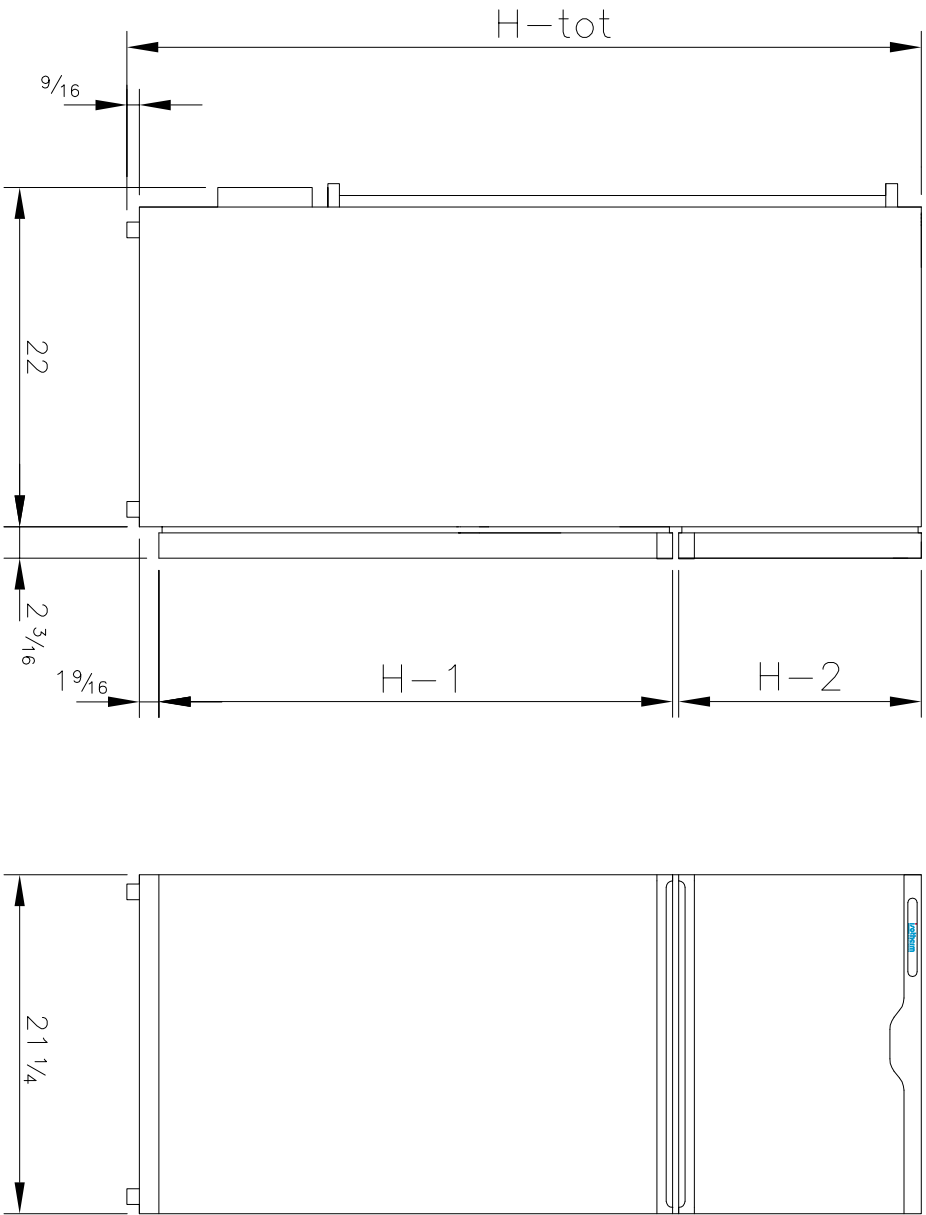
Installation dimensions
